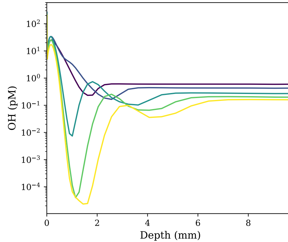
(e) OH
