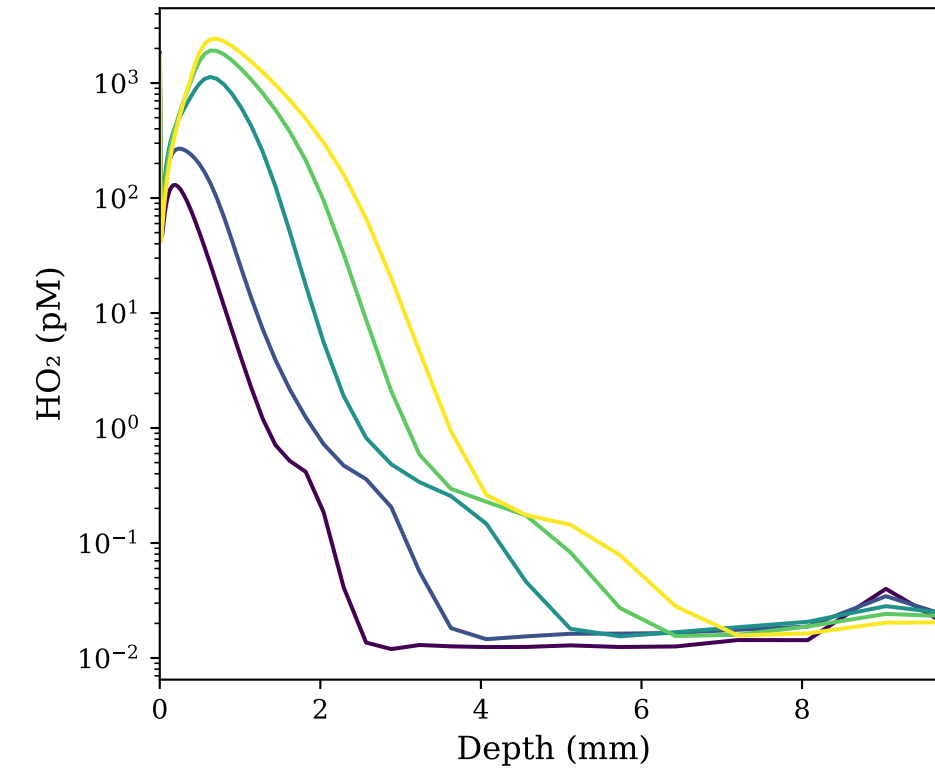
(f) \text{HO}_2
